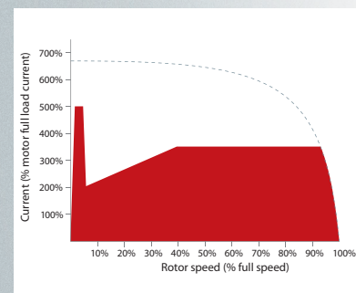
Constant current/ current ramp – shown here with kickstart
